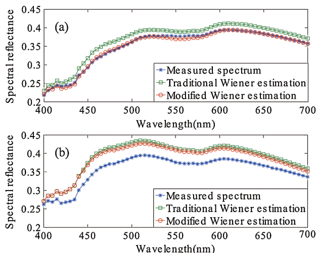
Fig. 4 Comparison between the measured diffuse reflectance spectrum and the spectrum estimated by the modified Wiener estimation method in the cases of (a) best estimation and (b) worst estimation. The results from traditional Wiener estimation are also shown for comparison.
