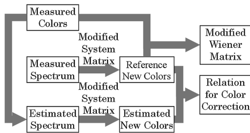
Fig. 1 Schematic of the calibration stage.
